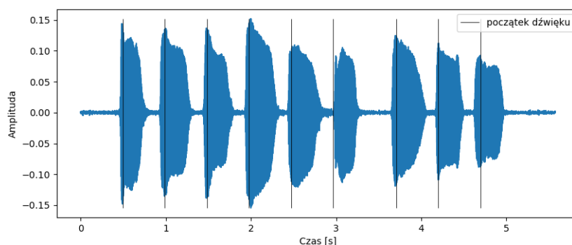
Rysunek 2.7: „Wlazi kotek na plotek v.1”, Short-term energy method n_0 = 5450 , threshold = 5
