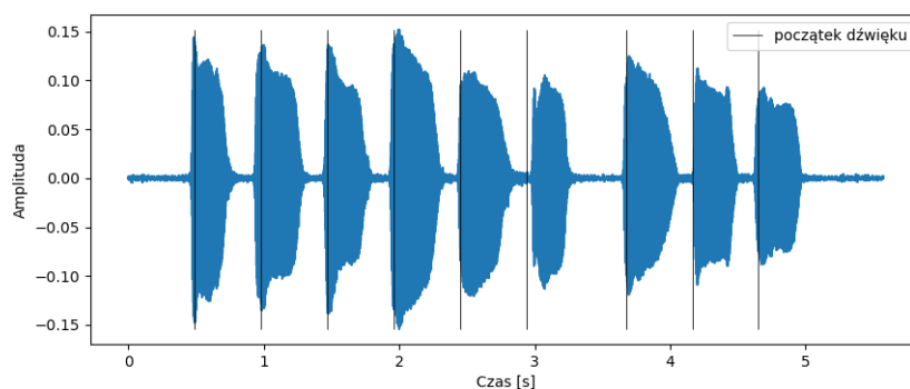
Rysunek 2.8: „Wlazi kotek na plotek v.1”, Short-term energy method n_0 = 5400 , threshold = 5 , \epsilon = 8000
