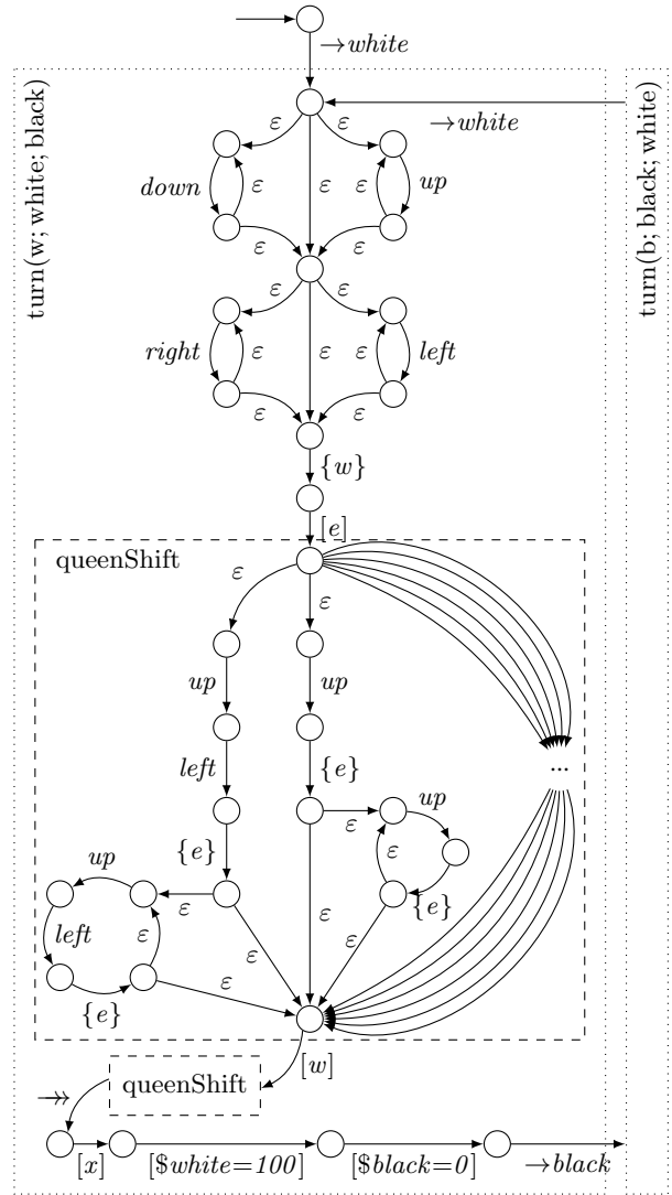
Fig. 2. NFA represented by the Amazons description from Fig.1.
